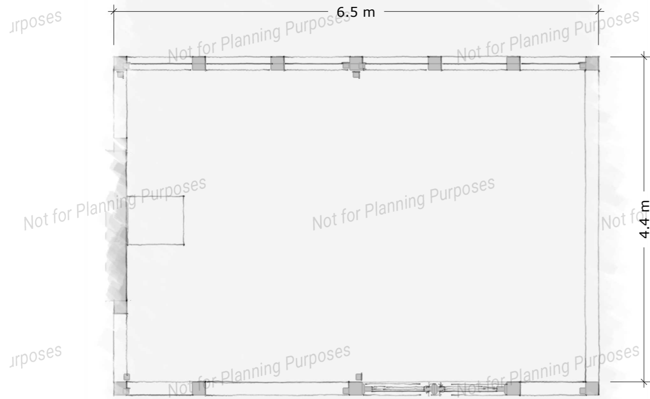
PLAN Scale 1:50
