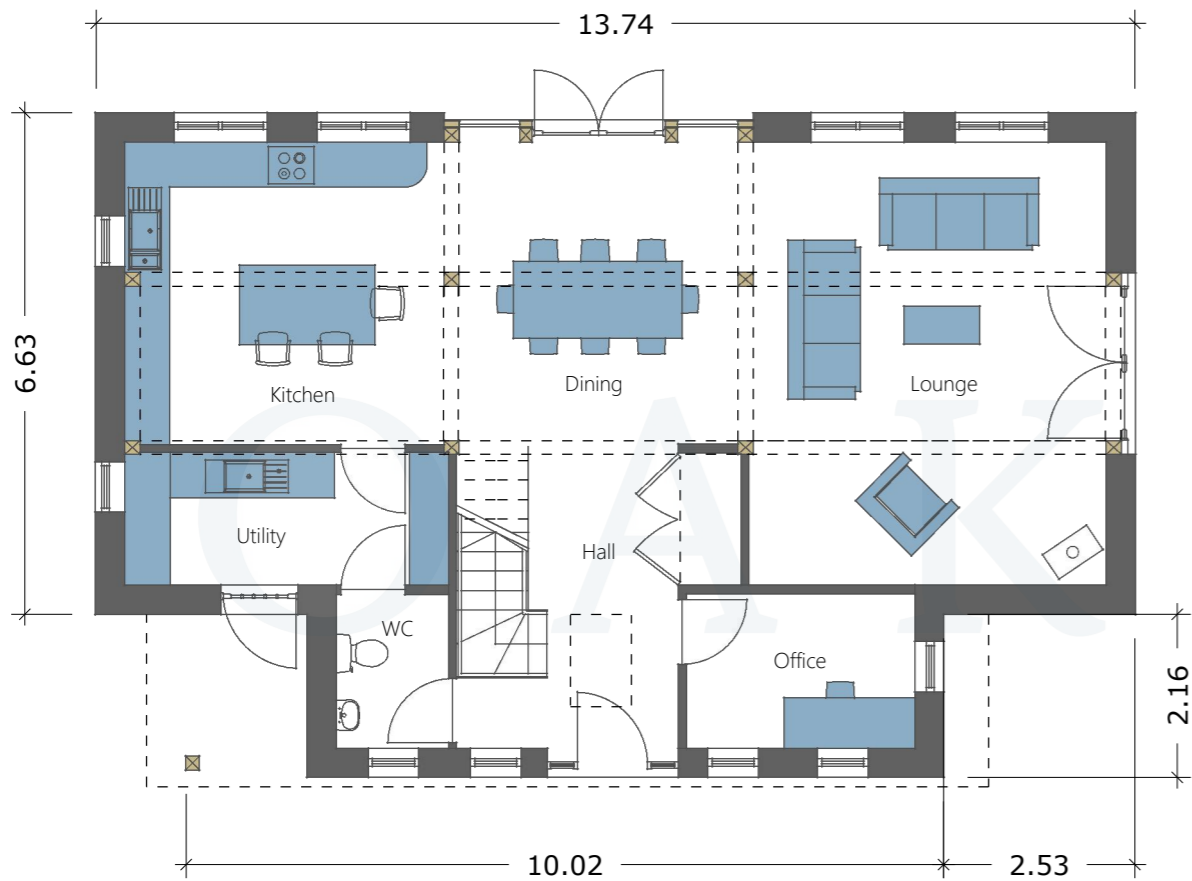
GROUND FLOOR GEA- 93.72m 2
