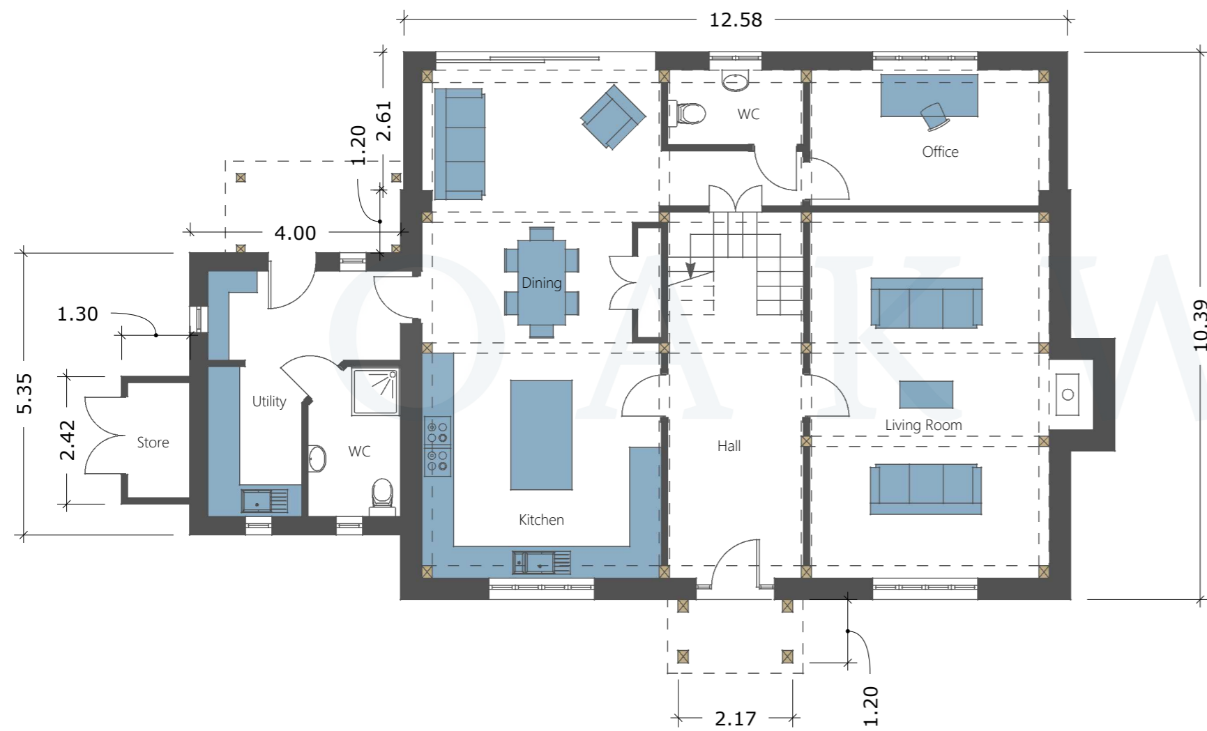
GROUND FLOOR GEA- 165.32 m 2
