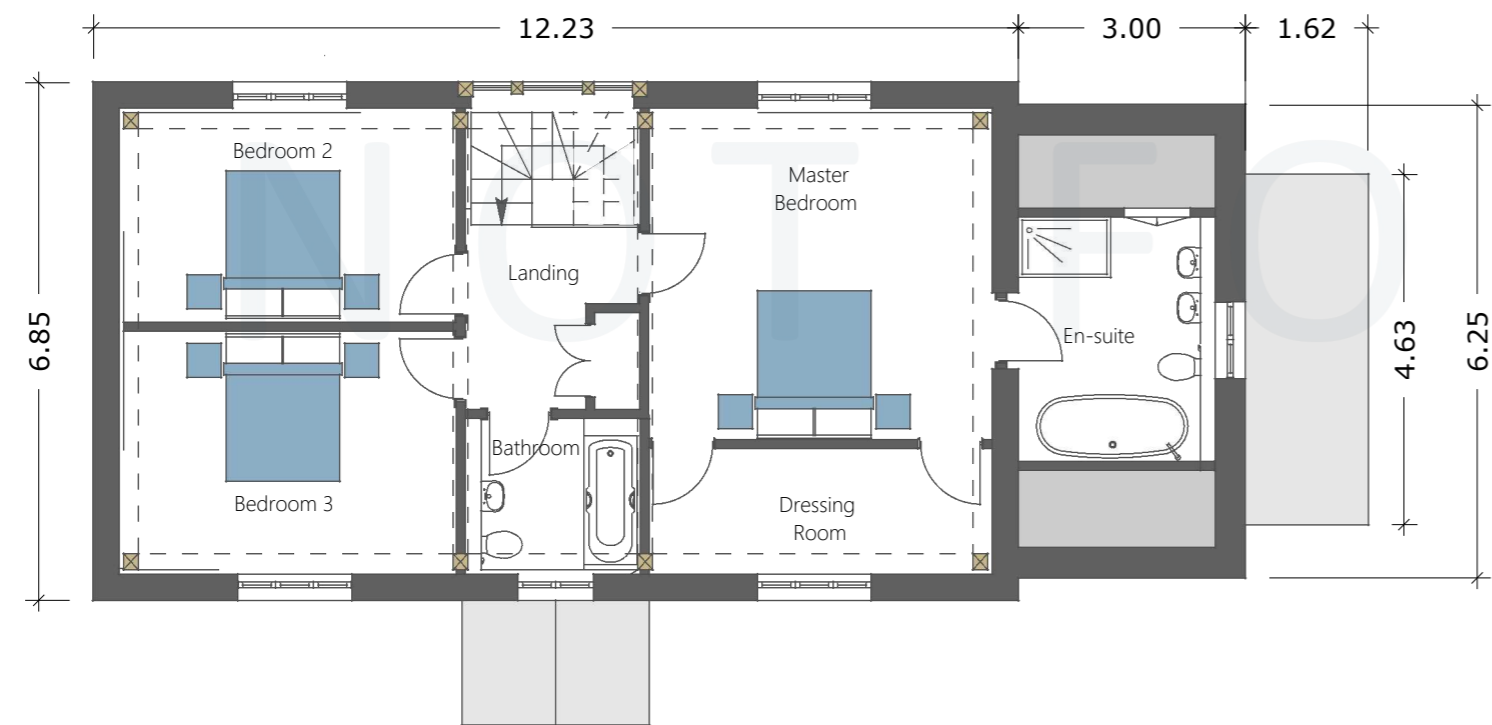
FIRST FLOOR GEA- 102.5 m 2
