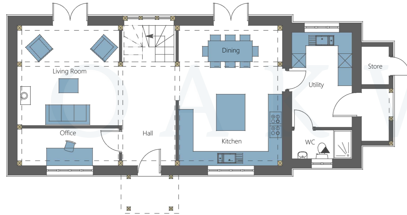
GROUND FLOOR GEA- 114.72 m 2
