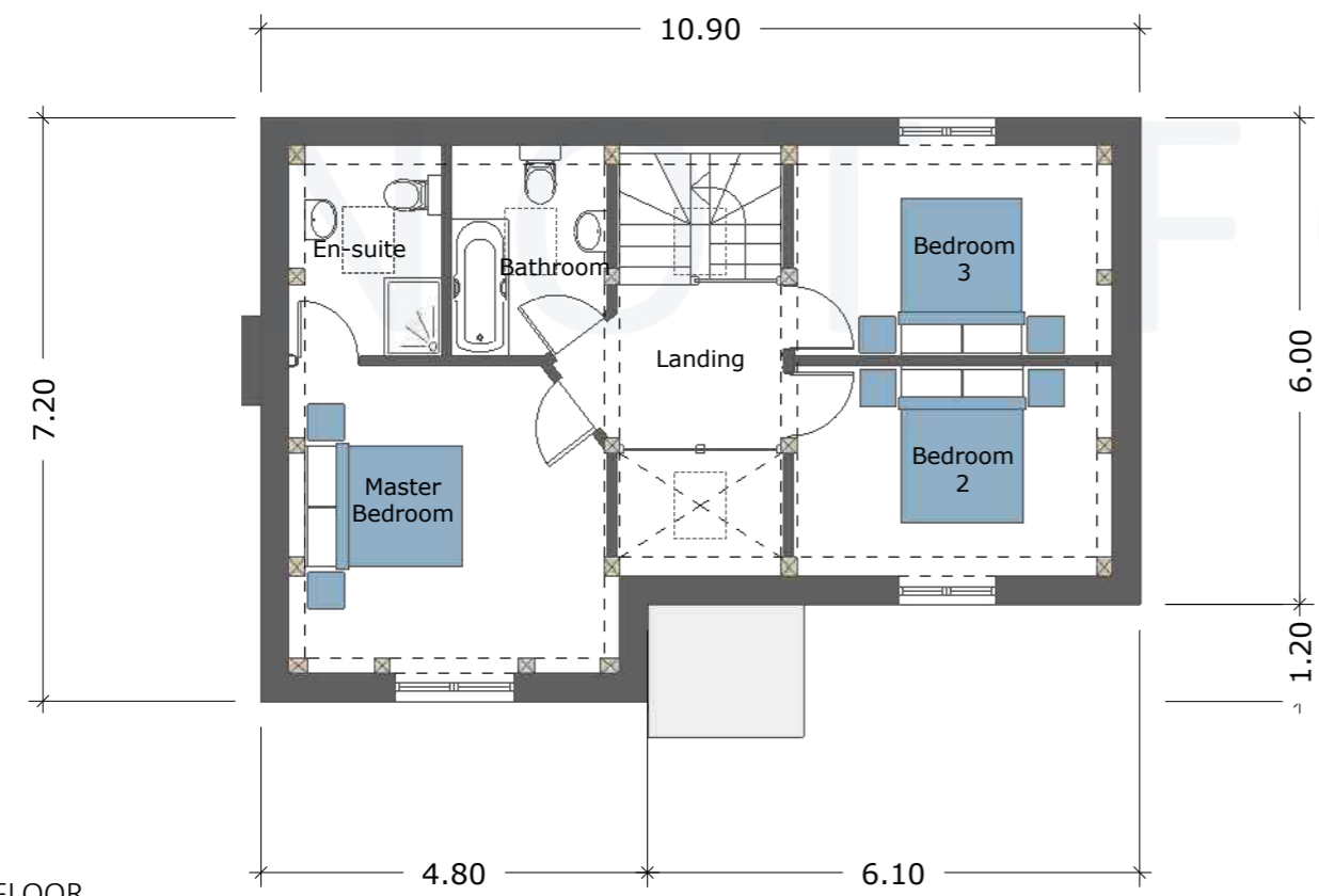
FIRST FLOOR GEA- 71.40m 2
