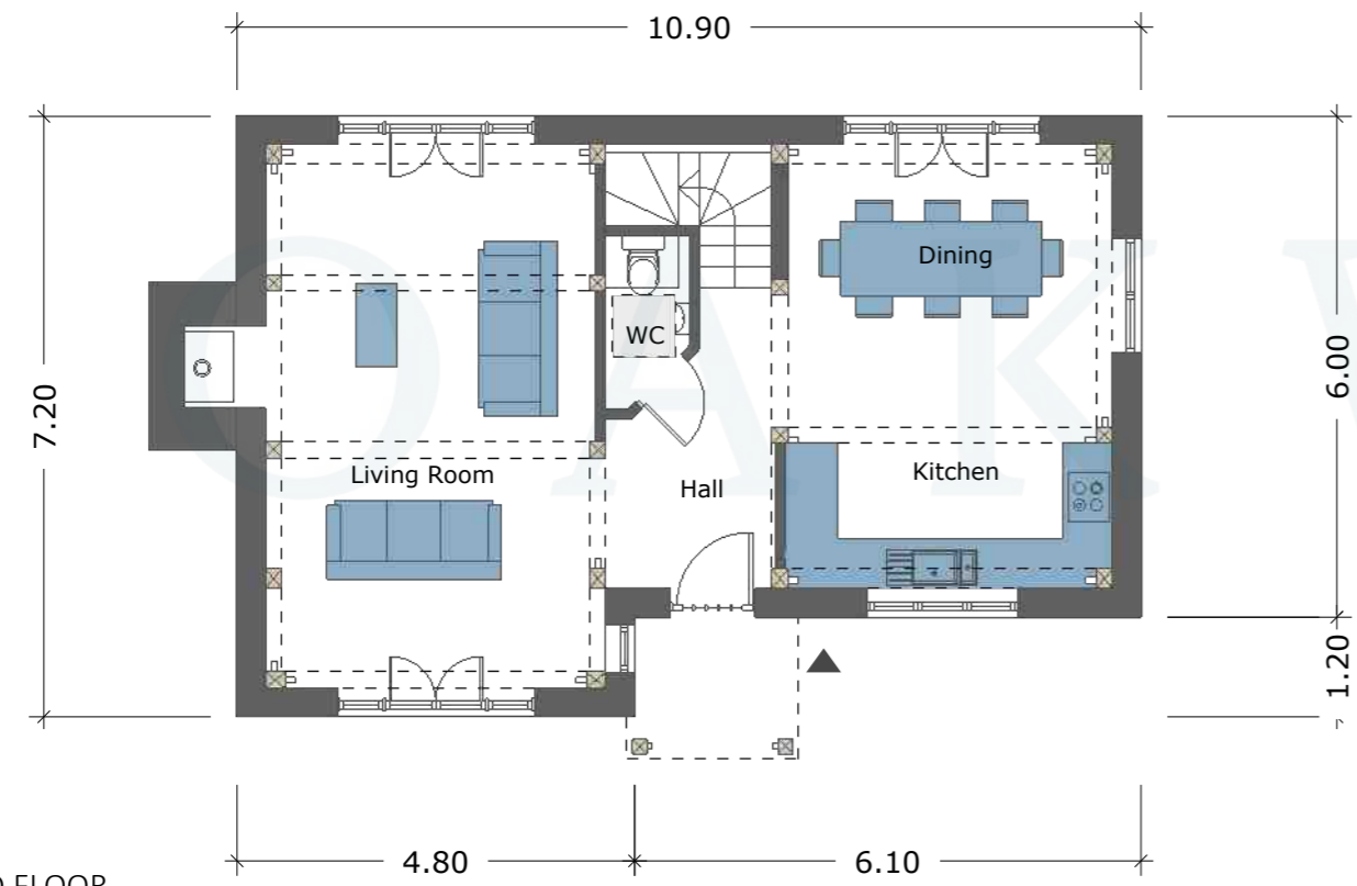
GROUND FLOOR GEA- 77.00m 2
