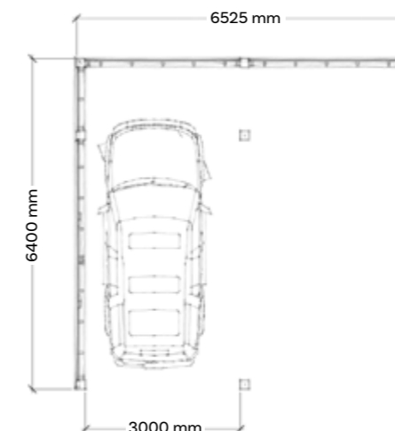
Floorplan
